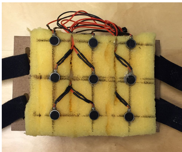
Fig. 2 The vibro-sponge with a 30-mm inter-tactor spacing (as used in experiment 1) and similar devices with an inter-tactor distance of 20 and 13 mm were used in experiments 2 and 3, respectively
